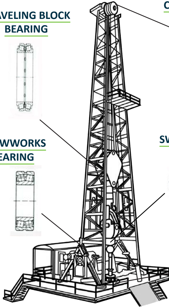
ROTARY RIG
